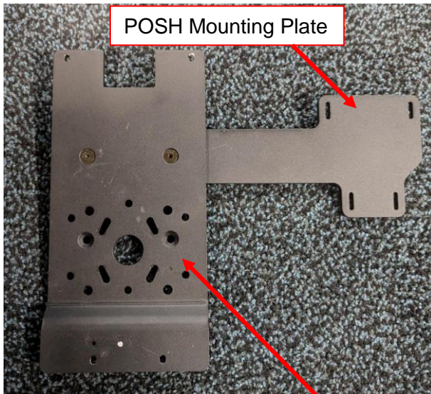
CF33 Laptop Mounting Plate
