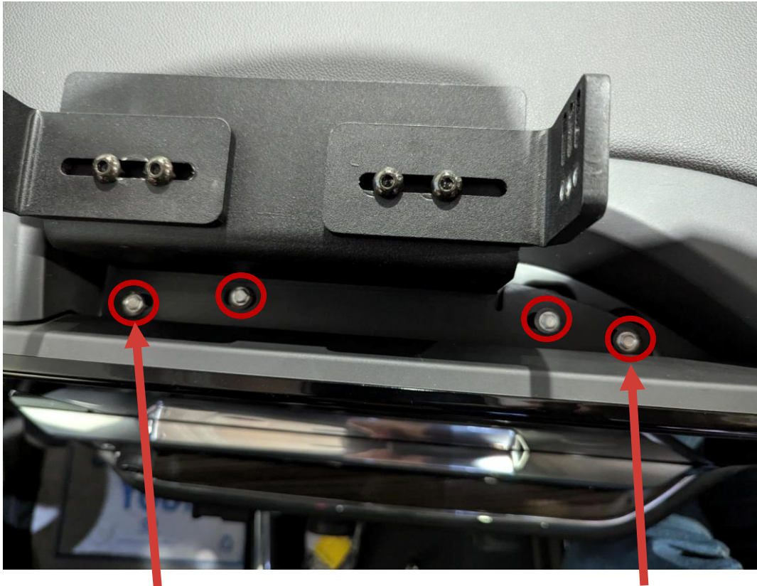
#8-15 X 1-1/2 Hex Head Screw
